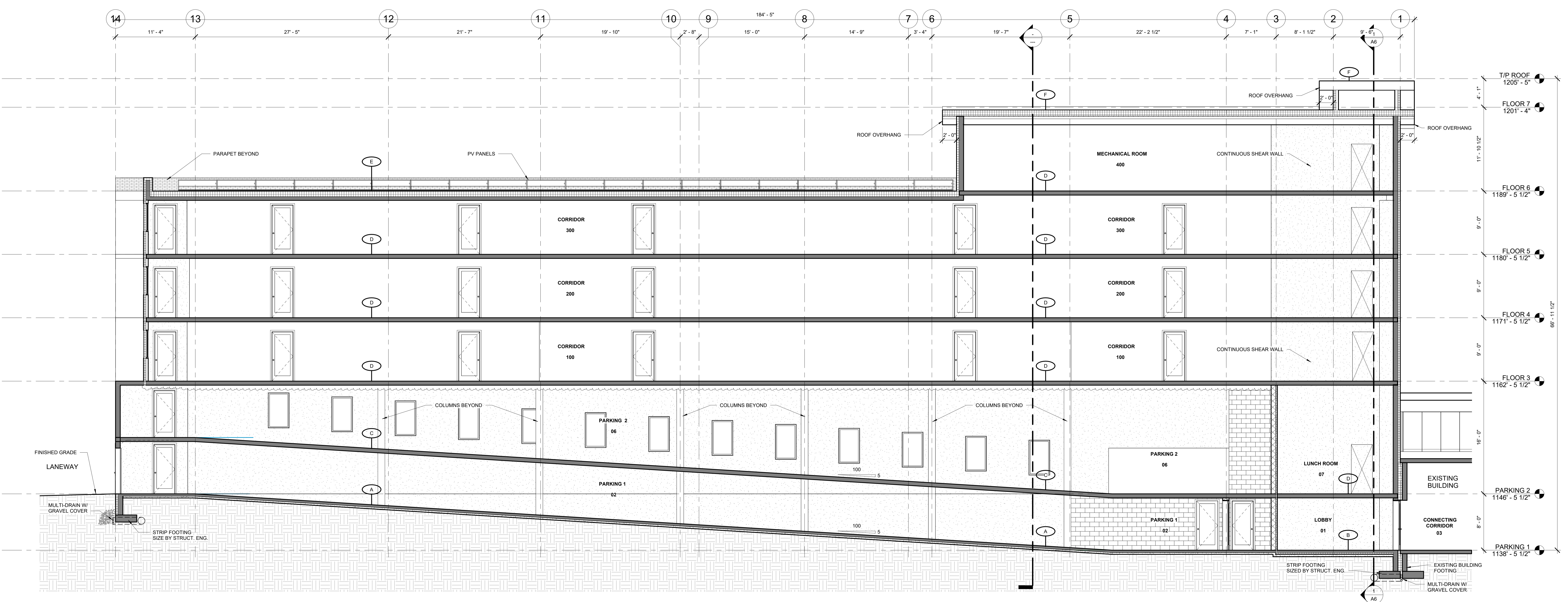
2 BUILDING SECTION 2 3/16" = 1'-0"
